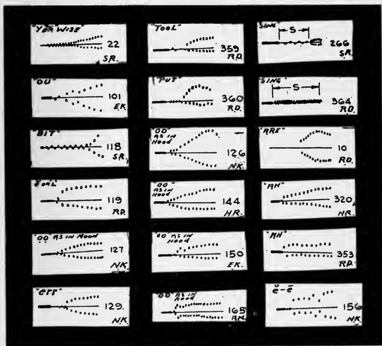
FIG. 2A. Tracings of oscillograms of Fig. 2.
